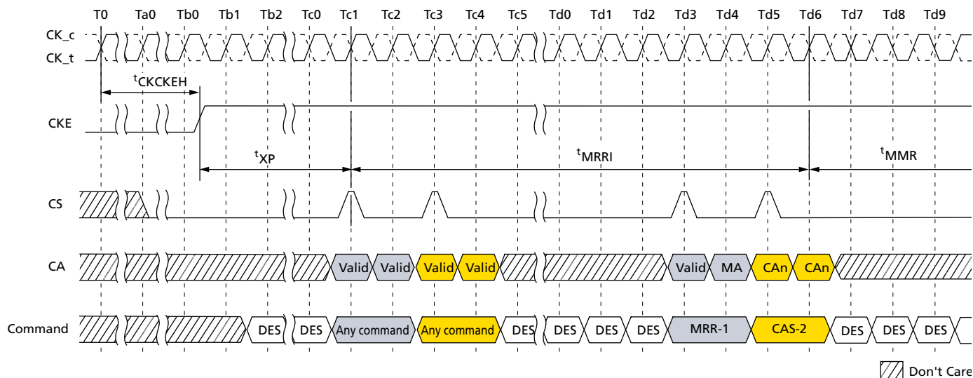
Figure 98: MRR Following Power-Down
