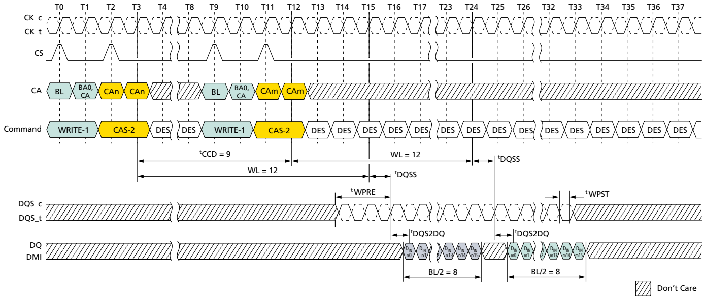
Figure 59: Consecutive WRITE: t_{CCD} = \text{MIN} + 1, 0.5nCK Postamble
