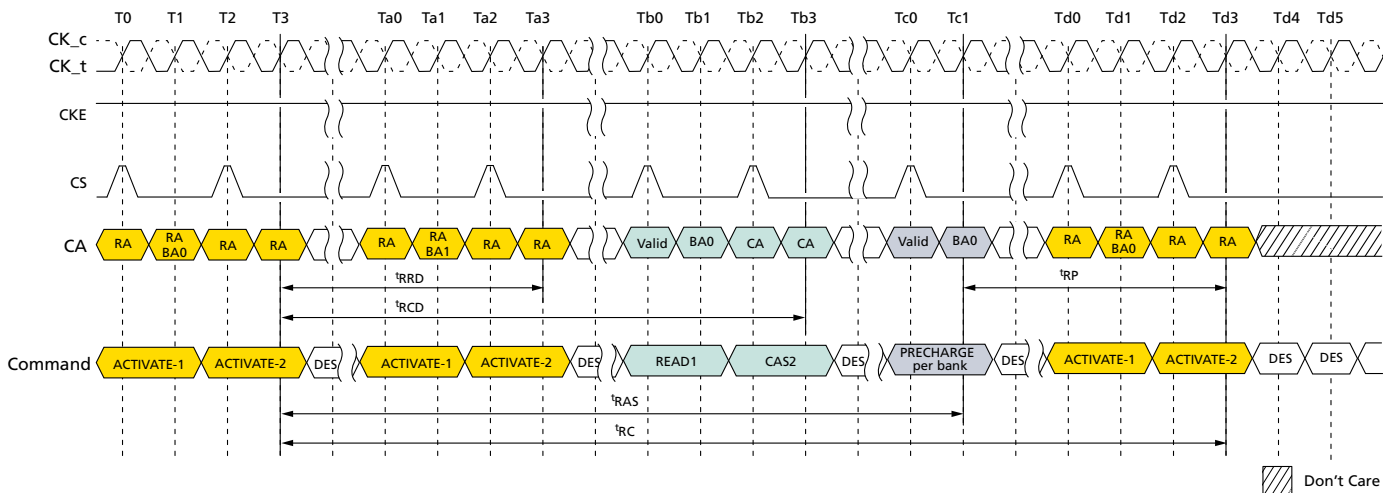
Figure 16: ACTIVATE Command
