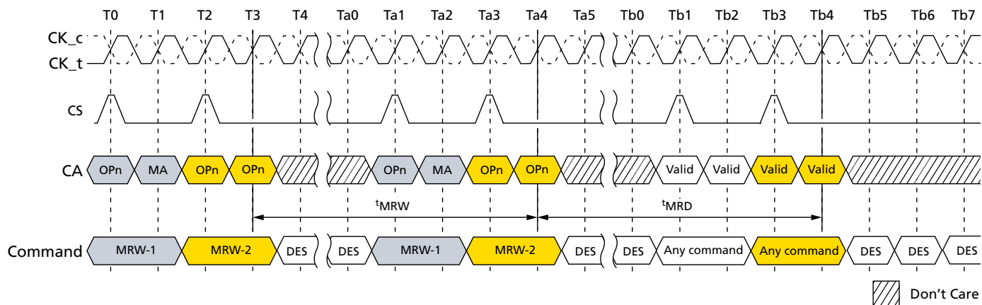
Figure 99: MODE REGISTER WRITE Timing
