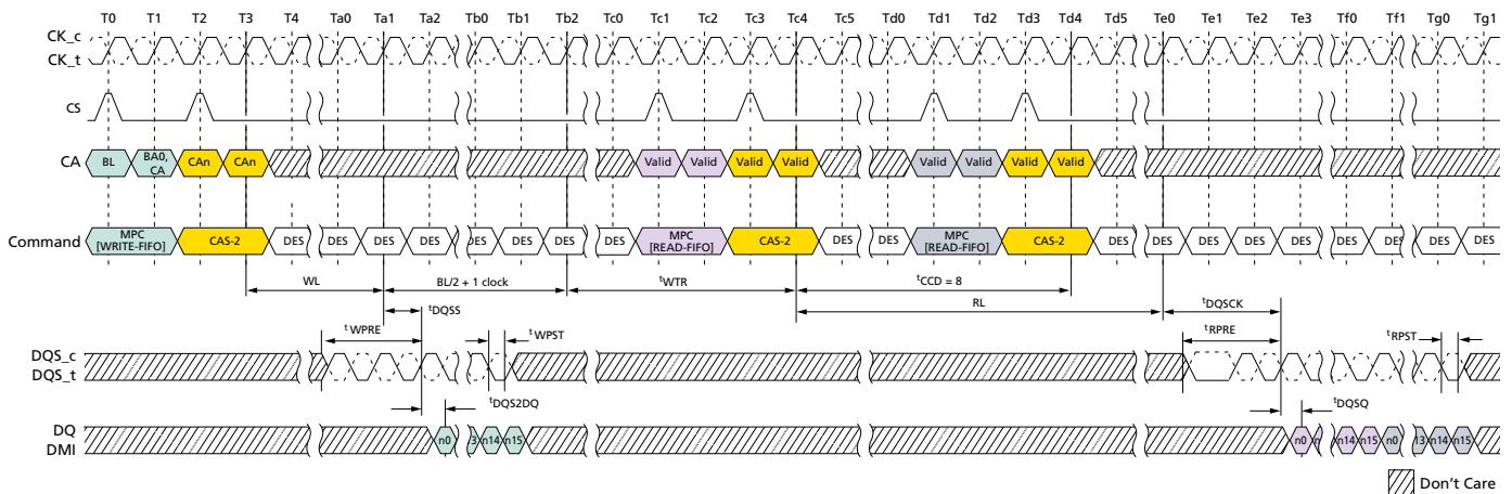
Figure 131: MPC[WRITE-FIFO]-to-MPC[READ-FIFO] Timing
