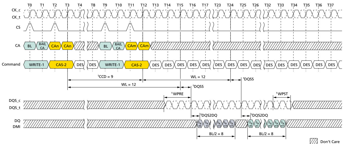
Figure 60: Consecutive WRITE: t_{CCD} = \text{MIN} + 1, 1.5nCK Postamble
