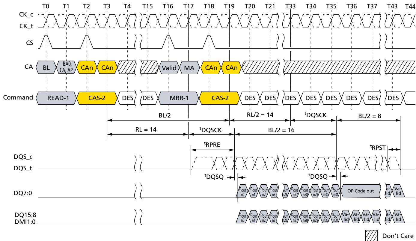
Figure 96: READ-to-MRR Timing
