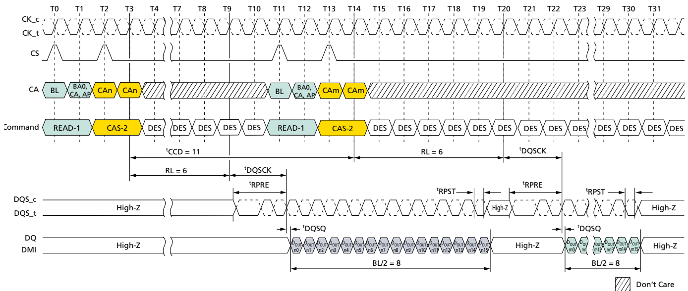
Figure 53: Consecutive READ: t_{CCD} = \text{MIN} + 3 , Preamble = Toggle, 0.5n\text{CK} Postamble
