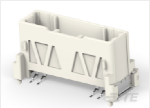
TE Part #1-2295435-1 36POS,HYBRID,HDR ASSY,180DEG, SMD
