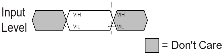
Figure 7.1b — Input AC timing definition for Reset_n and ODT_CA
