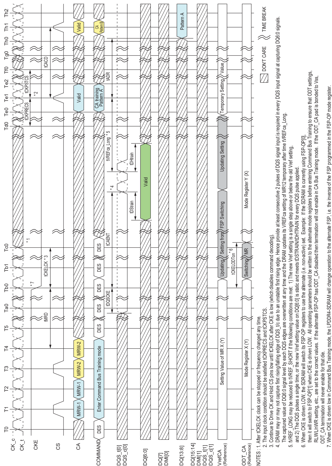
Figure 4.83— Entering Command Bus Training Mode and CA Training Pattern Input and Output with VREFCA Value Update
