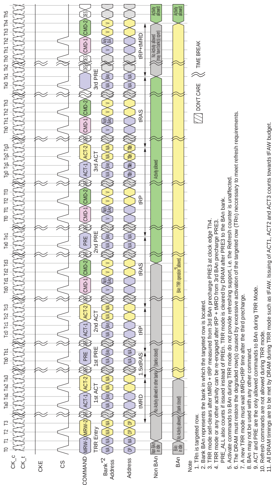
Figure 4.129 — TRR Mode
