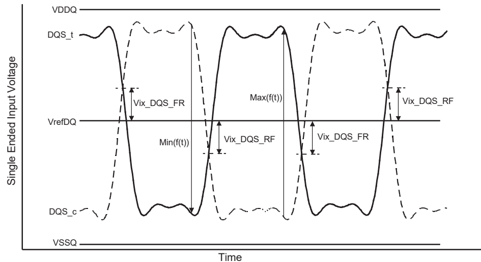
Figure 7.12 — DQS input Crosspoint voltage (Vix)
