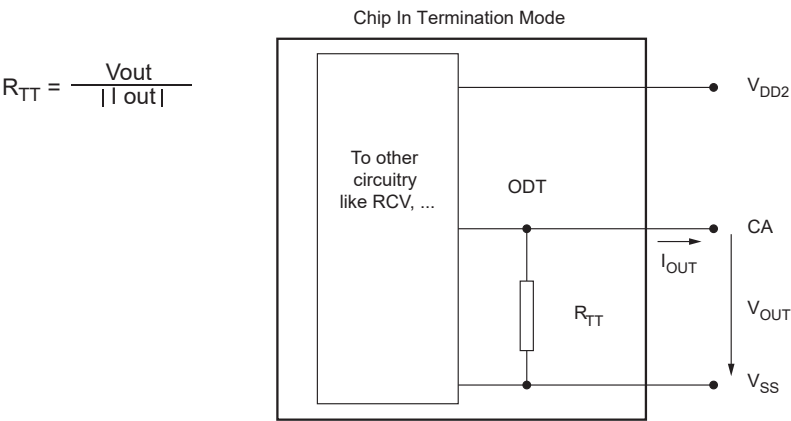
Figure 4.113a — On Die Termination for CA for LPDDR4
