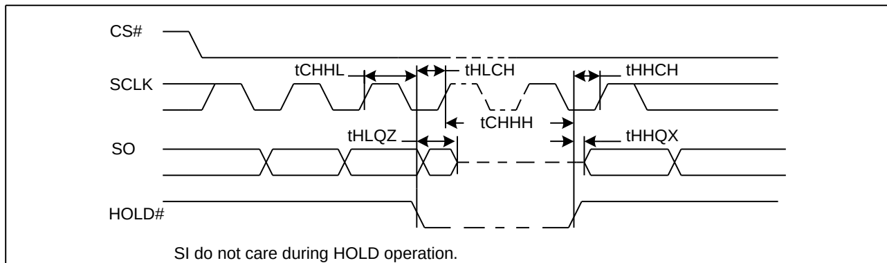
Figure 46. Hold Timing
