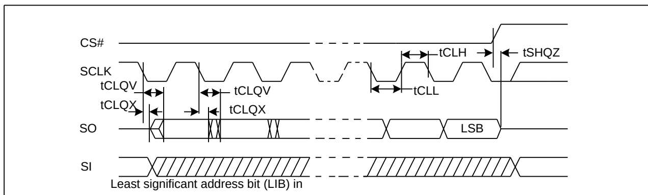
Figure 44. Output Timing
