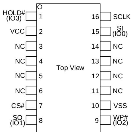
16-LEAD SOP
