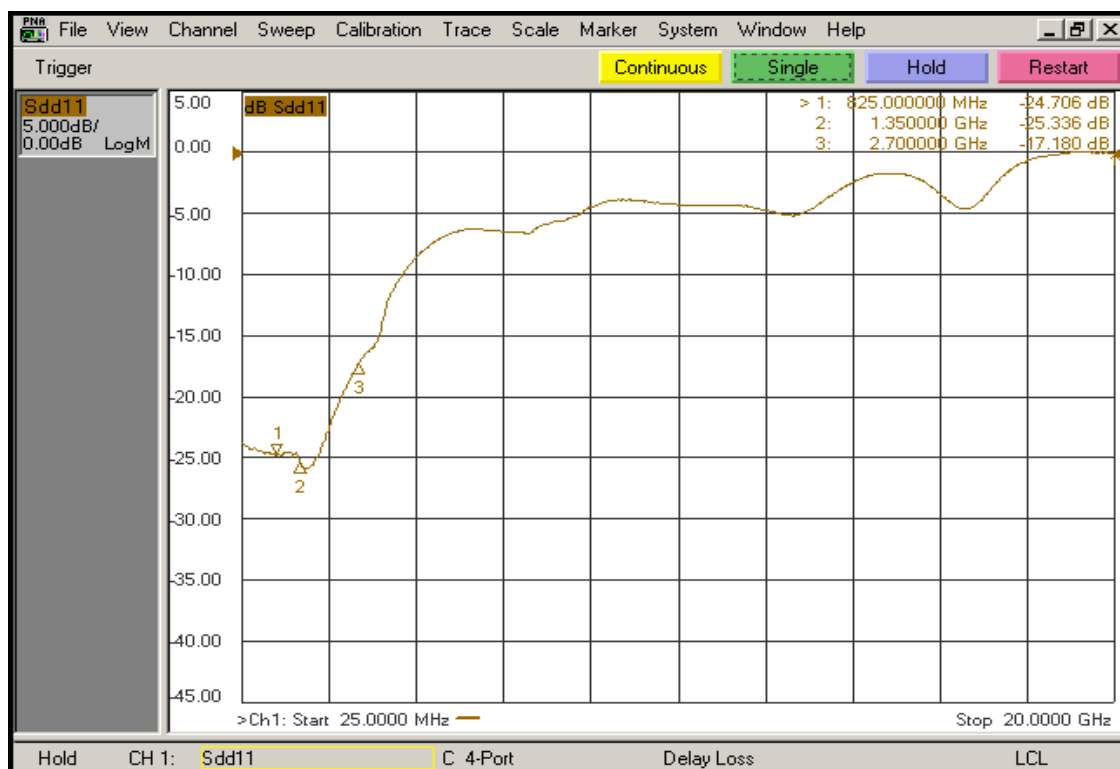
Figure 7. Return Loss
