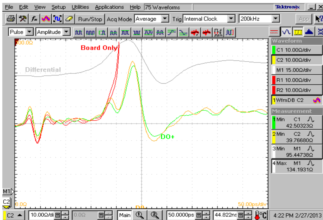
Figure 8. TDR Channel D0, VDD=3.0V, 25C
