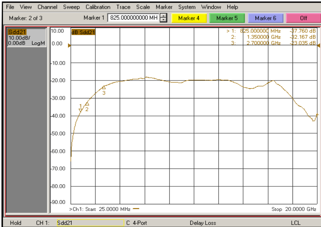
Figure 5. Off Isolation
