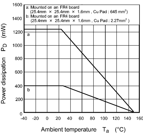
Fig. 8.13 P_D - T_a
