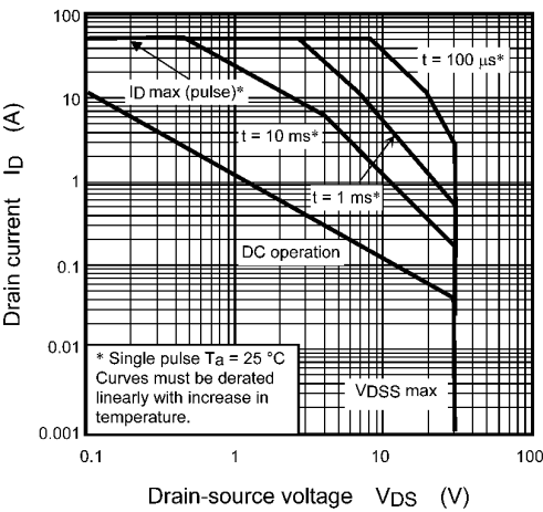
Fig. 8.14 Safe Operating Area
