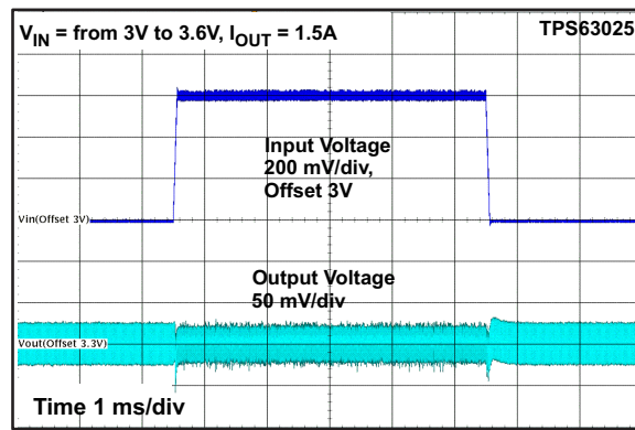
Figure 24. Line Transient Response
