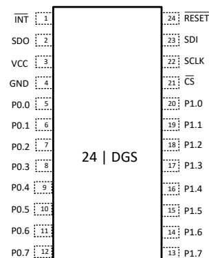
Figure 4-2. TXE8116 DGS (VSSOP) Package, 24-Pin (Top View)
