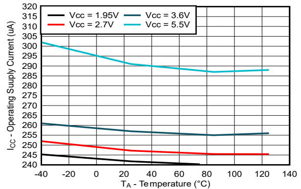
Figure 5-2. Operating Supply Current vs Temperature ( f_{\text{SCLK}} = 10\text{MHz} )
