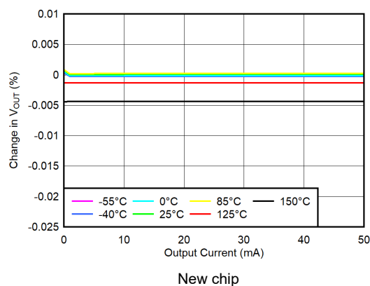
图 5-6. Load Regulation at Light Load
