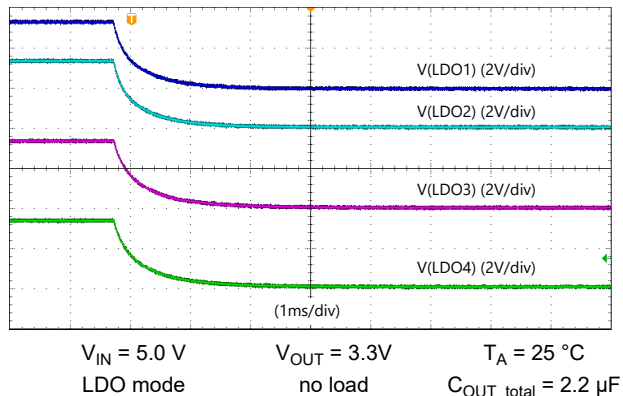
Figure 7-9. LDOs Discharge
