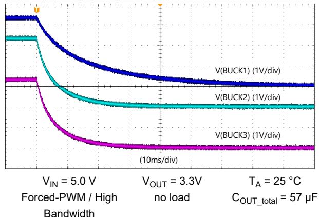
Figure 7-8. Bucks Discharge
