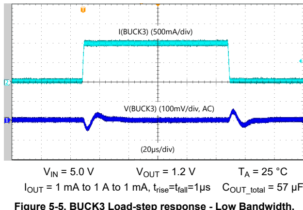
Figure 5-5. BUCK3 Load-step response - Low Bandwidth, forced PWM
