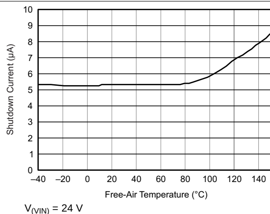
Figure 9. Shutdown Current
