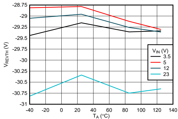
Figure 6-18. RCB - Reverse Comparator Threshold vs Temperature
