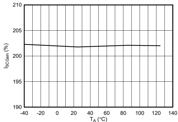
Figure 6-14. Steady State Scalable Fast-trip Threshold: Current Limit Threshold ( I_{LIM} ) Ratio vs Temperature (TPS259480x/2x)
