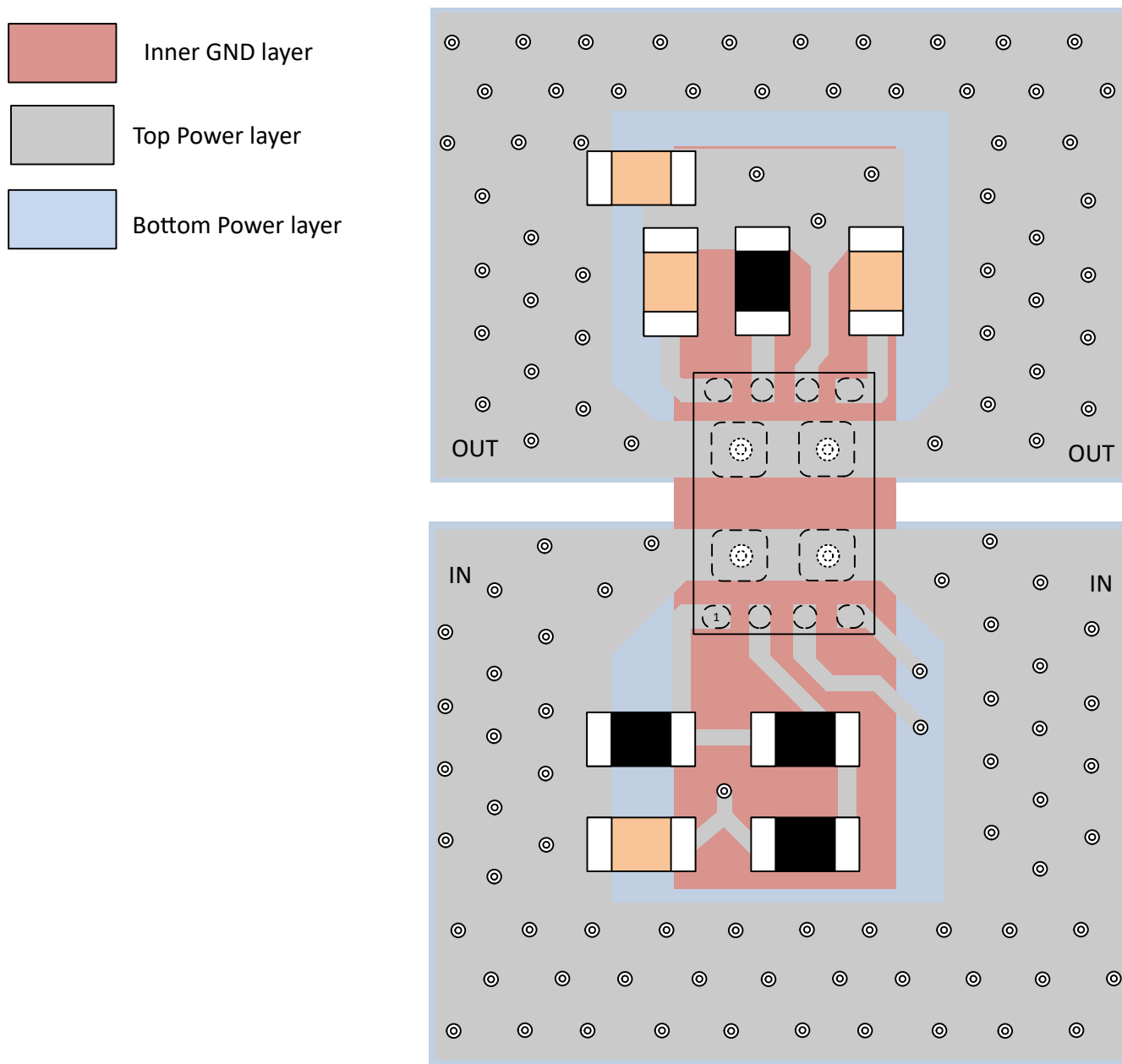
Figure 8-24. Layout Example
