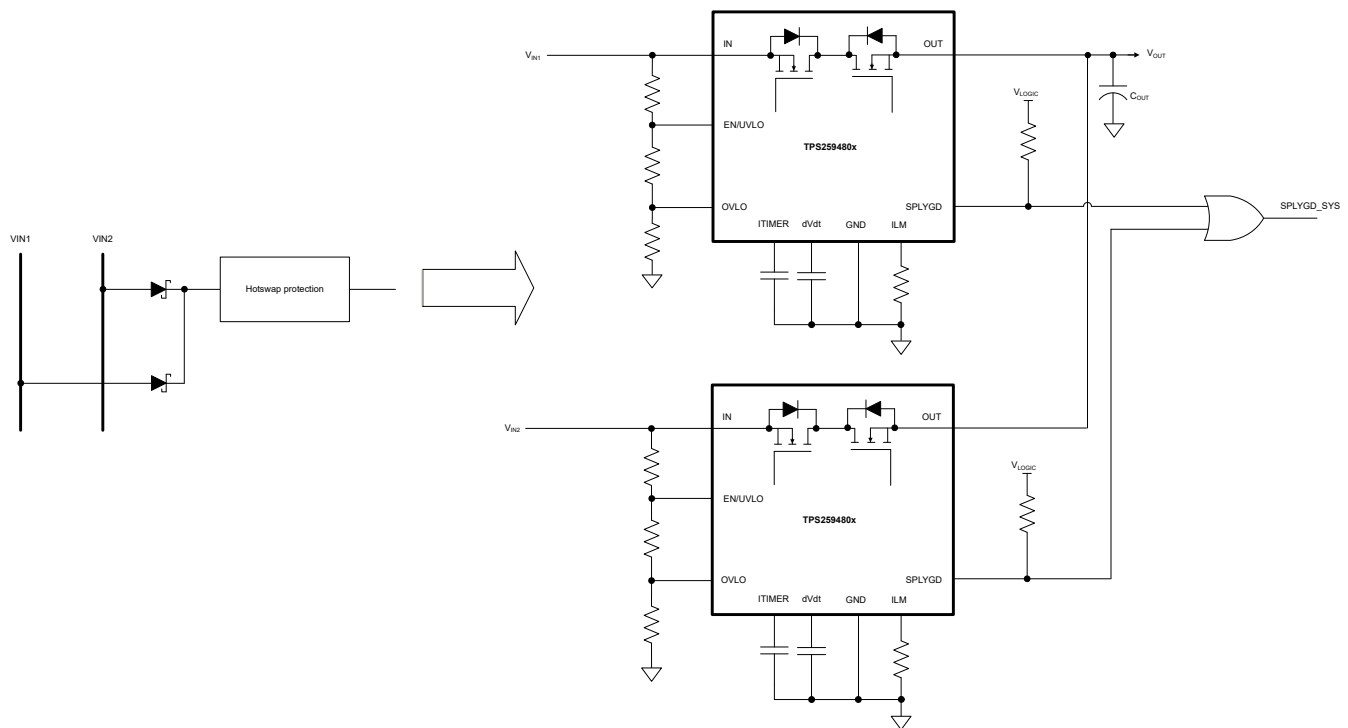
Figure 8-11. Two Devices, Active ORing Configuration
