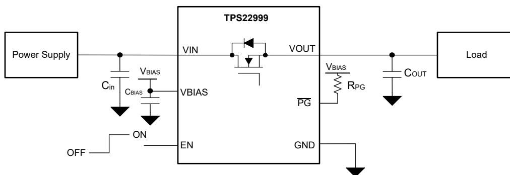
图 7-1. TPS22999 Basic Application
