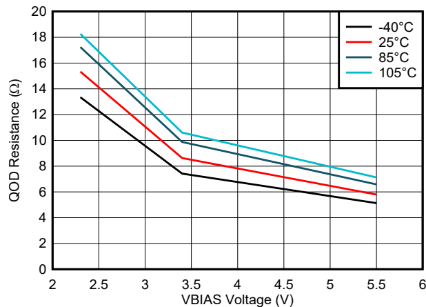
图 5-5. QOD Resistance vs VBIAS Voltage
