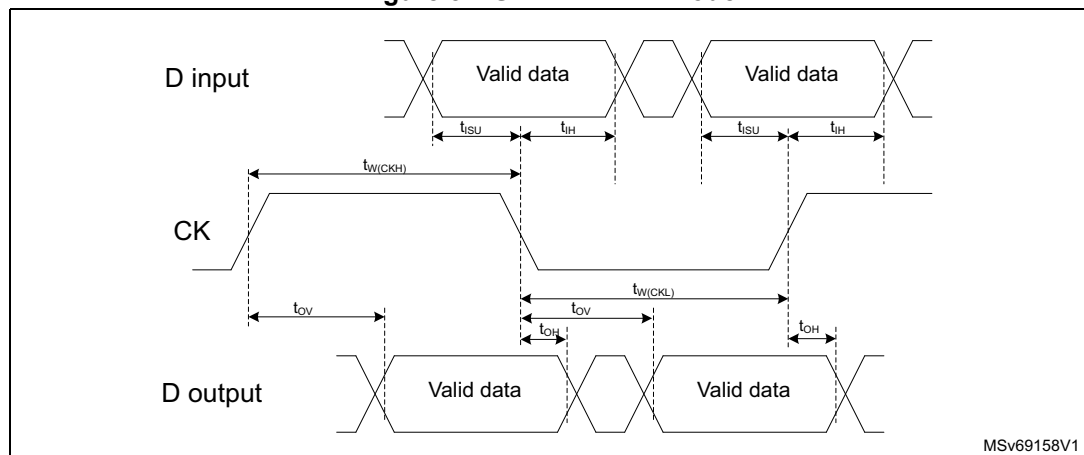
Figure 51. SDRAMC DDR mode
