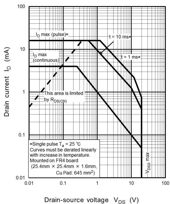
Fig. 7.13 Safe Operating Area
