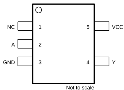
图 5-1. SN74AHC1G14-Q1 DBV Package, 5-Pin SOT-23; DCK Package, 5-Pin SC-70 (Top View)
