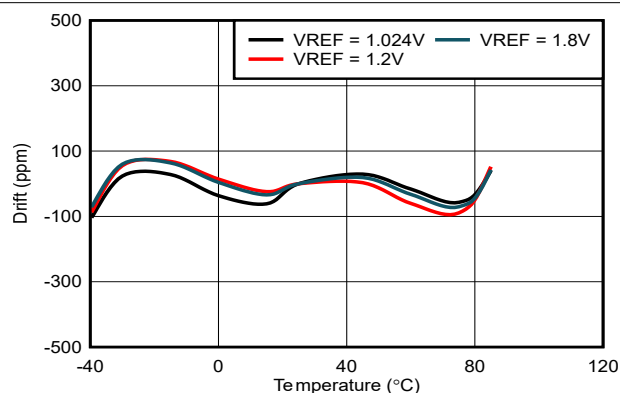
图 6-5. Output Voltage Drift vs Free-Air Temperature
