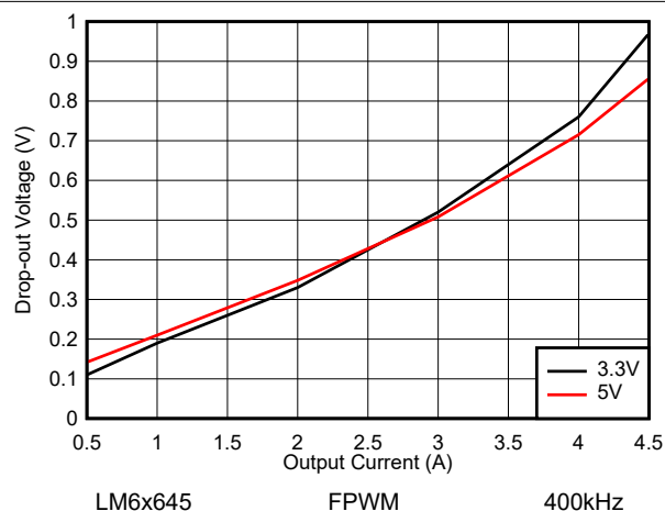
图 8-40. LM6x645 压降电压
