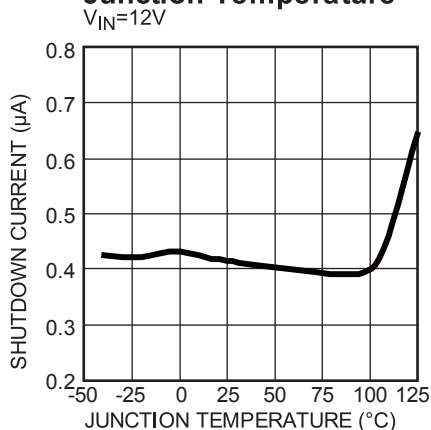
Shutdown Current vs. Junction Temperature V_{IN}=12V
