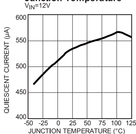
Quiescent Current vs. Junction Temperature V_{IN}=12V
