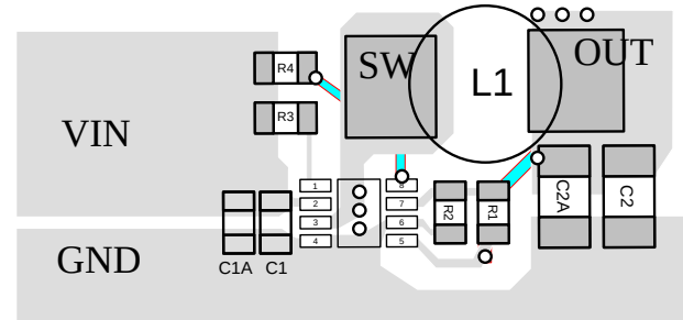
Figure 3: Layout Recommendation
