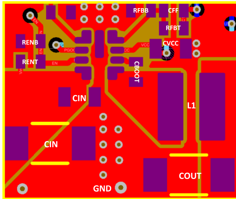
Figure 9-16. Example Layout
